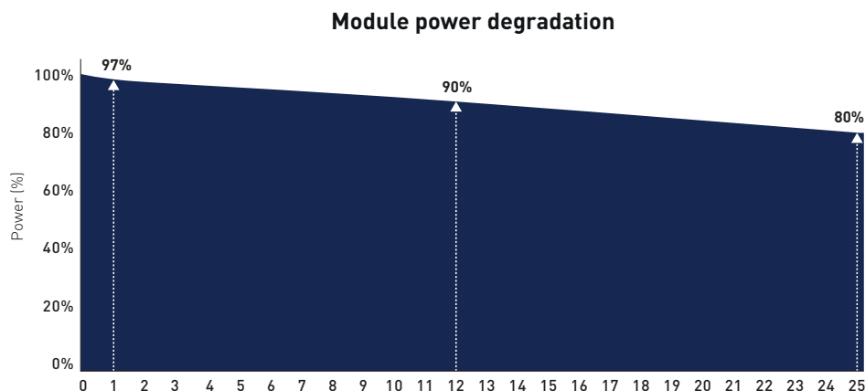
PICTURE 1. LINEAR POWER DEGRADATION GRAPH
