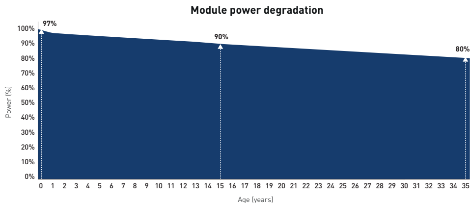
PICTURE 1. LINEAR POWER DEGRADATION GRAPH
